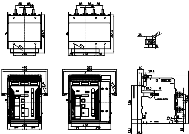
HGN(S) A06~16 VERTICAL EXTRAIBLE
