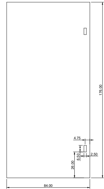
PUERTA INTERIOR
